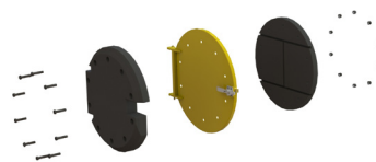
Impact Pad NPR02414-00
